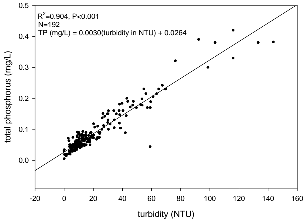
Turbidity and total phosphorus relationships for all mainstem Portneuf R and Marsh Cr sites*
